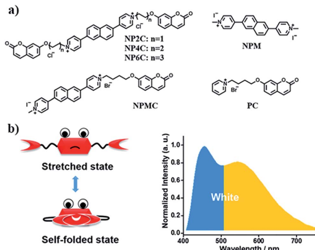
Fig. 1 (a) Molecular structures of white-light emitting organic molecules (NP4C and NP6C) and the reference compounds (NP2C, NPM, NPMC and PC); (b) the schematic cartoon illustration of single-molecule white-light emitters.
