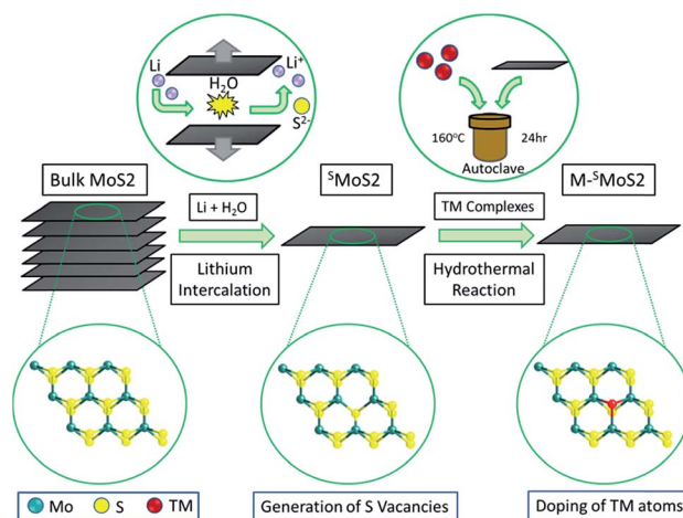
Fig. 1 Synthesis of single-layered MoS 2 ( S MoS 2 ) and single transition-metal (TM) atom doped F MoS 2 / S MoS 2 SO 4 2- groups.
