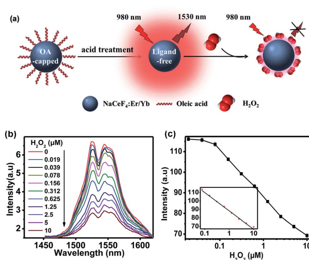
Fig. 3 (a) Process and principle of homogeneous assay of \text{H}_2\text{O}_2 by employing \text{NaCeF}_4\text{:Er/Yb} as the probe. (b) NIR-II emission spectra of ligand-free \text{NaCeF}_4\text{:Er/Yb} NCs after the addition of different concentrations of \text{H}_2\text{O}_2 upon excitation at 980 nm. (c) Calibration curve for the \text{H}_2\text{O}_2 assay. The inset shows the linear range ( 0.078\text{--}10 \mu\text{M} ) of the calibration curve.
