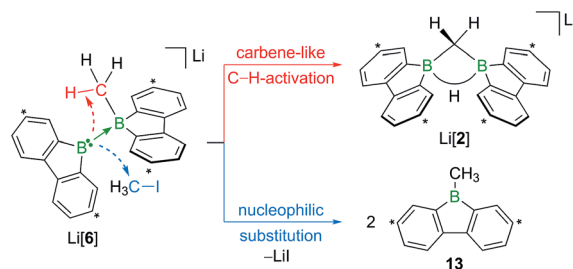
Scheme 9 The intermediate \text{Li}[6] can be interpreted as an adduct between the 9-borabiphenyl anion ( [\text{BFlu}]^- ) and 9-methyl-9-borabiphenyl ( 13 ). Intramolecular C-H insertion of the carbene-like [\text{BFlu}]^- furnishes \text{Li}[2] ; intermolecular nucleophilic attack on \text{H}_3\text{C-I} affords 2 equiv. of 13 . Carbon atoms marked with asterisks bear t Bu substituents.
