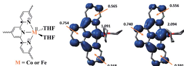
Fig. 7 Proposed electronic structure of \text{M}^{\text{II}}(\text{THF})_2 \cdot (\text{TPY}^{\bullet\bullet})^{2-}\text{-MOL} , \text{M} = \text{Co} or \text{Fe} (left); calculated Mulliken spin density distribution and spin density plots (blue: positive; green: negative) of \text{Co}(\text{tpy})(\text{THF})_2 quartet state (middle) and \text{Fe}(\text{tpy})(\text{THF})_2 quintet state (right).
