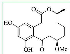
363: (11β)-11-methoxycurvularin
