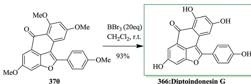
Scheme 77 Total synthesis of diptoindonesin G 366 .
