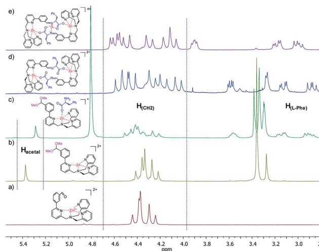
Fig. 2 Comparison of the ^1\text{H} -NMR signals for the compounds 1 , 4 , 5-L-Phe , 1-L-Phe and 2-L-Phe in \text{D}_3 -acetonitrile. In this region acetal (5.4 to 5.2 ppm), \text{CH}_2 picolil (4.6 to 3.9 ppm) and amino acid (3.8 to 2.7 ppm) proton signals are present. The counteranions are perchlorate.
