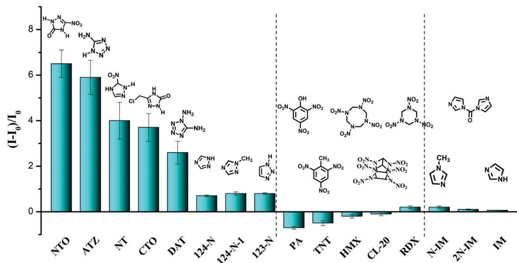
Fig. 3 Fluorescence enhancement ((I - I_0)/I_0) of E,E -HPB-ID by different analytes ( M_{E,E-HPB-ID} : M_{\text{analytes}} = 1 : 2 ) in the 90% water fraction in THF/water mixtures. [E,E\text{-HPB-ID}] = 1 \times 10^{-4} \text{ mol L}^{-1} .
