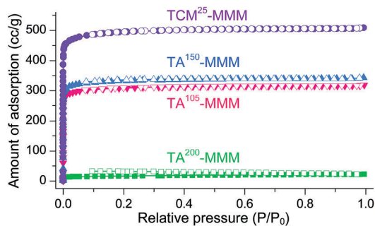
Fig. 19 N _2 adsorption/desorption isotherms of TA ^{105} -, TA ^{150} -, TA ^{200} -, and TCM ^{25} -MMM. The isotherms for the TCM ^{25} -MMM sample were measured after applying vacuum at room temperature for 4 h. Reprinted (adapted) with permission from ref. 70. Copyright (2018) American Chemical Society.
