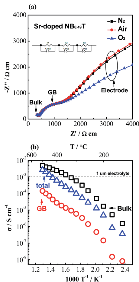
Fig. 3 (a) Complex impedance, Z^* , plots for 2% Sr-doped \text{NB}_{0.49}\text{T} with Pt electrodes under different atmospheres at 400^\circ\text{C} ; the inset figure is the equivalent circuit used to fit the impedance data. (b) Arrhenius plots for \sigma_b , \sigma_{\text{GB}} and \sigma_{\text{tot}} for 2% Sr-doped \text{NB}_{0.49}\text{T} . The horizontal dash line indicates the minimum conductivity requirement for a 1 \mu\text{m} electrolyte for SOFCs. 8
