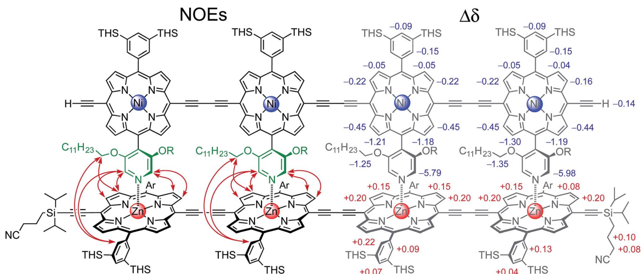
Fig. 2 The chemical structure of the 4-rung ladder complex NiP4·CPDIPS-ZnP4 (CDCl 3 , 500 MHz, 298 K) together with key NOEs between the components (left) and complexation-induced changes in proton chemical shift.
