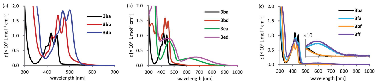
Fig. 1 UV-vis absorption spectra of (a) 3ba , 3bb , and 3db , (b) 3ba , 3bd , 3ea , and 3ed , and (c) 3ba , 3fa , 3bf , and 3ff in \text{CH}_2\text{Cl}_2 ( 1.0 \times 10^{-4} \text{ M} ) at 25^\circ \text{C} .
