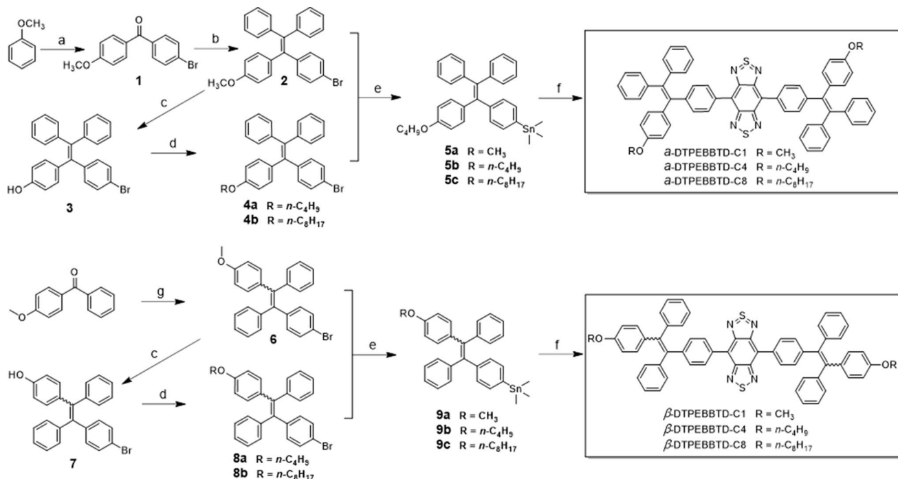
Scheme 1 Chemical structures and synthetic routes to \alpha -DTPEBBTD- C_x and \beta -DTPEBBTD- C_x . x represents the carbon numbers of the alkoxy chains on the TPE blocks, and x = 1, 4 or 8 . Reagents and conditions: (a) \text{AlCl}_3 , 4-bromobenzoyl chloride, \text{CH}_2\text{Cl}_2 , 0-10^\circ\text{C} , overnight; (b) (i) \text{BuLi} , diphenylmethane, 0^\circ\text{C} , overnight; (ii) p -toluenesulfonic acid, toluene, 100^\circ\text{C} , 3 h; (c) \text{BBr}_3 , \text{CH}_2\text{Cl}_2 ; (d) \text{Cs}_2\text{CO}_3 , DMF, room temperature, 1-bromobutane for 4a and 8a, 1-bromooctane for 4b and 8b; (e) \text{BuLi} , \text{Me}_3\text{SnCl} , THF, -78^\circ\text{C} , overnight; (f) \text{Pd}(\text{PPh}_3)_4 , toluene, 100^\circ\text{C} , 24 h.
