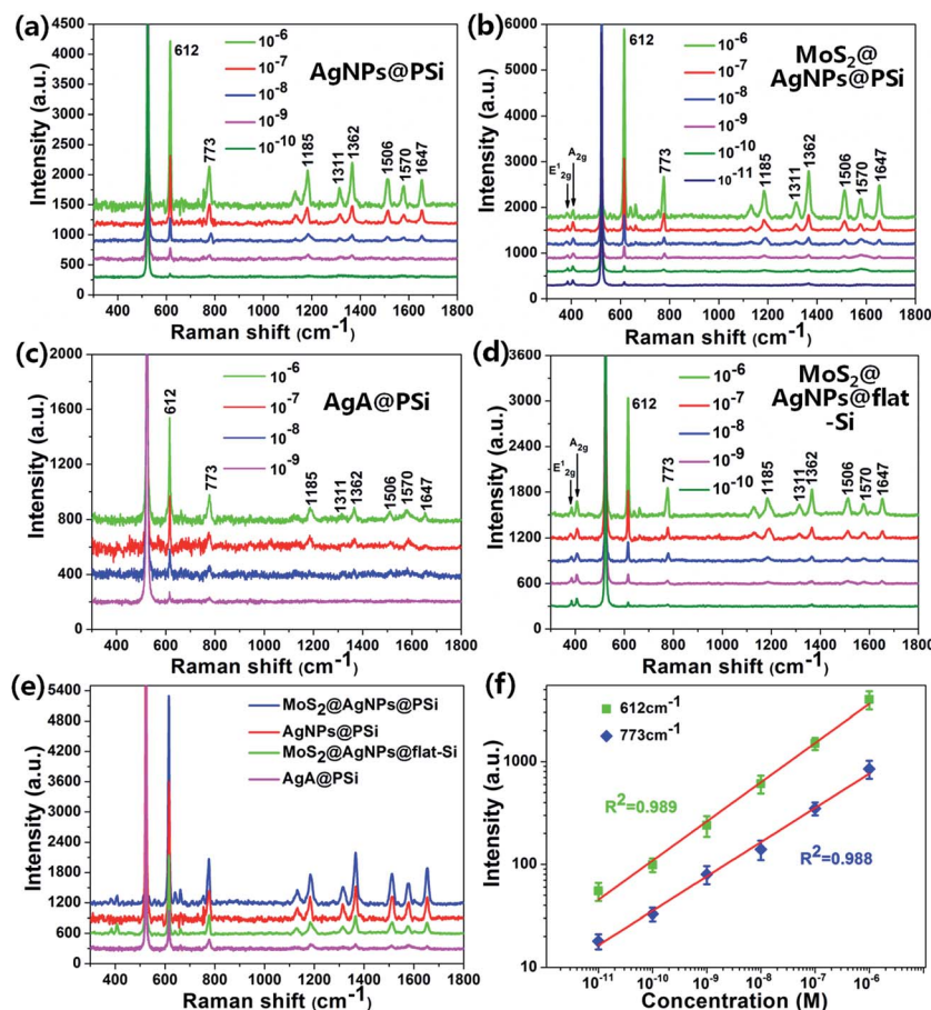
Fig. 5 (a) The Raman spectra of R6G on the AgNPs@PSi substrate from 10^{-6} to 10^{-10} M. (b) The Raman spectra of R6G on the \text{MoS}_2\text{@AgNPs@PSi} substrate from 10^{-6} to 10^{-11} M. (c) The Raman spectra of R6G on the AgA@PSi substrate from 10^{-6} to 10^{-9} M. (d) The Raman spectra of R6G on the \text{MoS}_2\text{@AgNPs@flat-Si} substrate from 10^{-6} to 10^{-10} M. (e) The Raman spectra of R6G on the \text{MoS}_2\text{@AgNPs@PSi} , AgNPs@PSi, \text{MoS}_2\text{@AgNPs@flat-Si} and AgA@PSi substrates with concentration of 10^{-6} M. (f) Raman intensity of R6G at 612 and 773 \text{cm}^{-1} as a function of the molecular concentration on the \text{MoS}_2\text{@AgNPs@PSi} substrate, in log scale.
