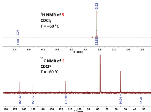
Fig. 1 ^1\text{H} NMR and ^{13}\text{C} NMR spectra of 5 .
