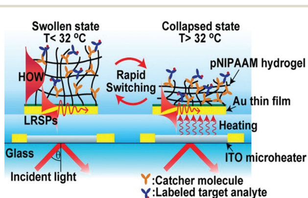
Fig. 1 Schematic diagram of a pNIPAm- co -MAAc hydrogel modified SPR sensor device with embedded ITO microheaters enabling rapid signal tuning. Reprinted with permission from ref. 67. Copyright 2013, American Chemical Society.
