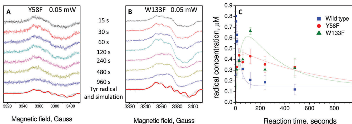
Fig. 3 EPR analysis of the formation and decay of the Tyr25 radical in wild type and variant BFR proteins. (A) Tyr58Phe BFR and (B) Trp133Phe BFR. Samples were 8.3 \mu M in 100 mM MES pH 6.5 frozen at variable times (as indicated) after addition of 72 \text{Fe}^{2+} per 24-mer. The tyrosyl radical spectrum obtained using the methodology of spectral subtraction as described in ref. 31 is shown in grey along with that simulated for the reported sidechain conformation of Tyr25, in each case the spectra are scaled according to the intensity observed 120 seconds after the addition of \text{Fe}^{2+} . Spectra were obtained at 10 K with the following instrumental conditions: microwave frequency = 9.467 GHz, microwave power = 0.05 mW, modulation frequency = 100 kHz, modulation amplitude = 3 G, scan rate = 0.596 \text{G s}^{-1} , time constant \tau = 82 ms. (C) Plots of tyrosyl radical concentrations versus time following addition of 72 \text{Fe}^{2+} per BFR 24-mer. The error bars principally represent uncertainties resulting from the method of spectral subtraction with variable coefficient used to deconvolute each spectrum into two spectral components and to determine their respective concentrations. 23 The data for the wild-type protein are from ref. 24. Data for the radicals are fitted to an \text{A} \rightarrow \text{B}^{\bullet} \rightarrow \text{C} kinetic scheme as discussed in the text.
