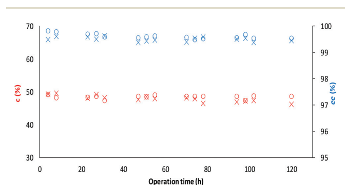
Fig. 8 Long term stability of the CaLB entrapped in the TDP sol-gel system in KR of the alcohol rac-1a ( c %; x, ee_{(R)-2a} %; o) and amine rac-3a ( c %; x, ee_{(R)-4a} %; o) in a continuous-flow reactor (60 °C, flow-rate of 0.1 mL min -1 ).
