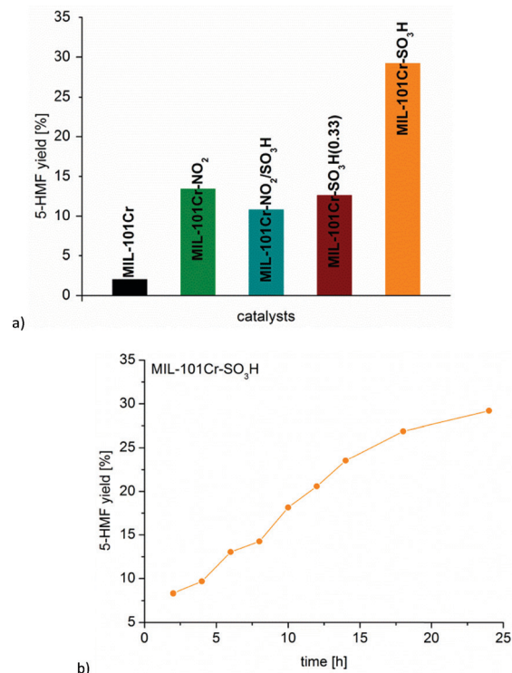
Fig. 21 (a) 5-HMF yield from glucose with different MIL-101Cr catalysts. (b) Time-dependent conversion for MIL-101Cr-SO 3 H (glucose 223 mg, 1.24 mmol, catalyst 5.22 × 10 -5 mol, 5 mL THF/H 2 O v:v 39:1, 130 °C, 24 h). Reprinted from ref. 134. Copyright 2016 with permission from the Royal Society of Chemistry.
