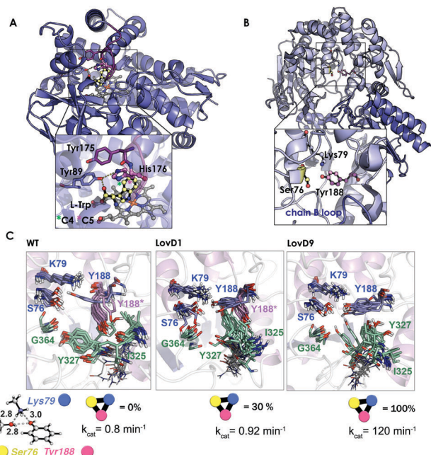
Fig. 7 (A) Homology model of the nitrating cytochrome P450 TxtE (PDB code: 4TPO). The F/G loop is highlighted in purple, and haem, L-tryptophan and His176 are represented by balls and sticks. (B) X-ray structures for the wild-type LovD enzyme (PDB code: 3HL9). (C) Optimized quantum mechanics arrangement of the catalytic triad, Lys79 is represented as a blue sphere, Ser76 as yellow, and Tyr188 as pink. Overlay of 10 snapshots from the ANTON MD simulations for wild-type enzyme in the monomeric state; LovD1 and LovD9 together with the computed percentage of time that the catalytic triad stays in the proper arrangement for catalysis along the MD trajectory. The experimental k_{\text{cat}} values (in \text{min}^{-1} ) are also included.
