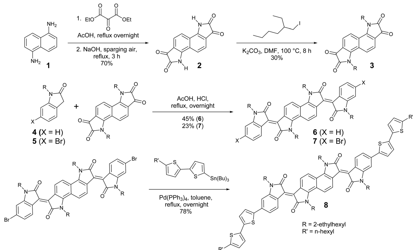
Scheme 1 Synthesis of bisoindigo (6) and bis(5'-hexyl-2,2'-bithienyl)-bisindigo (8).
