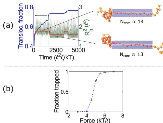
Fig. 3 Stick-slip motion of knotted polymers at intermediate forces. (a) Trajectory of a 4_1 -knotted polymer under constant force ( f = 5 kT/\ell ). When the motion stalls, the knot's radius of gyration makes a distinct hop. The red line is a piece-wise constant fit to the radius of gyration. Right: Snapshots of the knot show that the number of monomers in the knotted core changes during stick-slip motion. The bead size is equal to the rod length ( b = \ell ), but the beads are drawn small for illustrative purposes. (b) Fraction of time a knot is trapped as a function of force for the 4_1 topology. We consider a knot trapped if it moves less than 0.4\ell for times greater than 250 \ell^2 \zeta / kT . The data points are averages over 20–50 runs.
