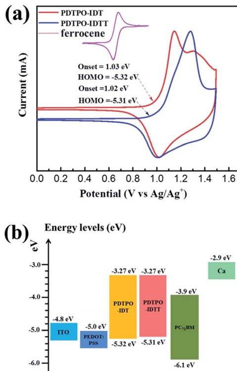
Fig. 2 (a) The electrochemical cyclic voltammetry measurements of PDTPPO-IDT and PDTPPO-IDTT thin film coated on the platinum electrode in acetonitrile solution containing 0.1 \text{ M } n\text{-Bu}_4\text{NPF}_6 at a scan rate of 100 \text{ mV s}^{-1} . (b) Schematic energy level diagram of all components used in conventional devices.
