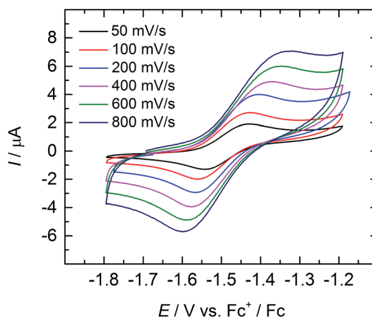
Fig. 5 Quasi-reversible oxidation wave of 3 at different scan rates. Measurement conducted in THF with \sim 0.1 M [\text{N}(n\text{-Bu})_4][\text{BPh}_4] electrolyte, using Fc + /Fc couple as internal standard.
