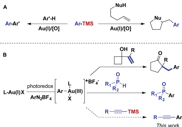
Scheme 1 Photoredox catalyst and visible light-mediated Au I /Au III catalysis.
