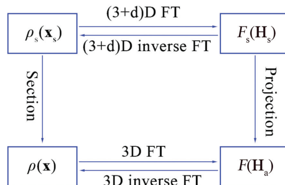
Fig. 4 The relationship between the electron density and structure factors is given by Fourier transform (FT) in the 3D or (3+d) D space.
