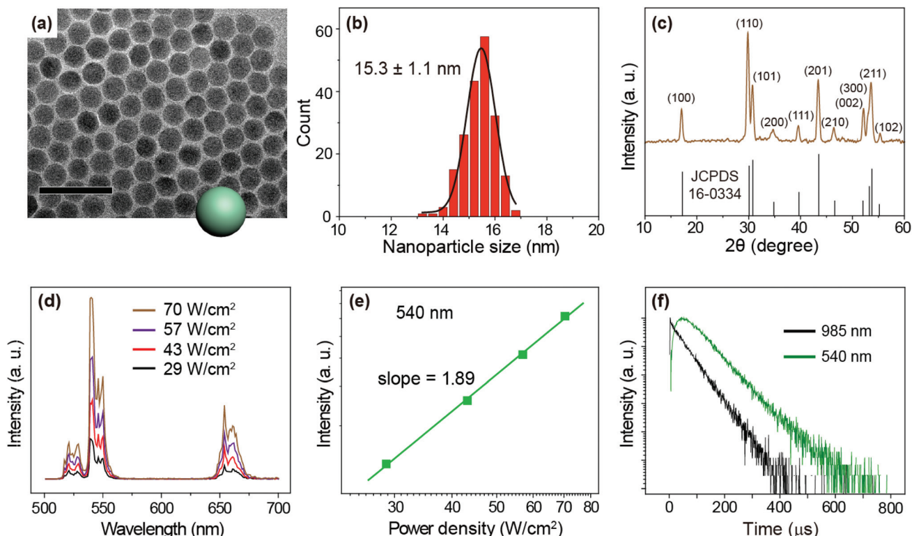
Fig. 2 (a) A typical TEM image of the as-prepared \text{NaYF}_4\text{:Yb/Er} (20/2%) nanoparticles. Scale bar is 50 nm. (b) Size histogram of the nanoparticles. (c) X-ray diffraction patterns of the nanoparticles, which are in good agreement with the literature reference for hexagonal \text{NaYF}_4 crystal (Joint Committee on Powder Diffraction Standards file number 16-0334). (d) Emission spectra of the UCNPs recorded with a 975 nm CW laser excitation at different power densities (29–70 \text{W cm}^{-2} ). (e) The 540 nm ( ^4\text{S}_{3/2} \rightarrow ^4\text{I}_{15/2} transition of \text{Er}^{3+} ) emission intensity versus pump power density in double-logarithmic representation. (f) Decay curves of 540 nm emissions from \text{Er}^{3+} as well as 985 nm from \text{Yb}^{3+} obtained upon excitation of the nanoparticles at 975 nm.
