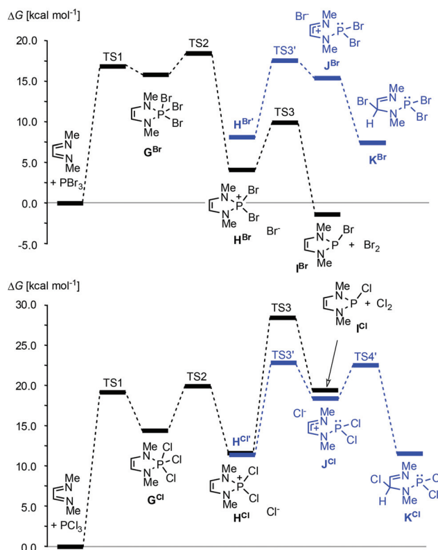
Fig. 4 Calculated minimum free energy pathways for the reactions of \text{MeN}=\text{CH}-\text{CH}=\text{NMe} with \text{PBr}_3 (top) and \text{PCl}_3 (bottom) at the B3LYP/def2-tzvp level. Solvent effects were modelled using a PCM approach. \text{H}^{\text{X}} and \text{H}^{\text{X'}} (X = Br, Cl) denote contact ion pairs with different ion arrangements. Data from ref. 36.
