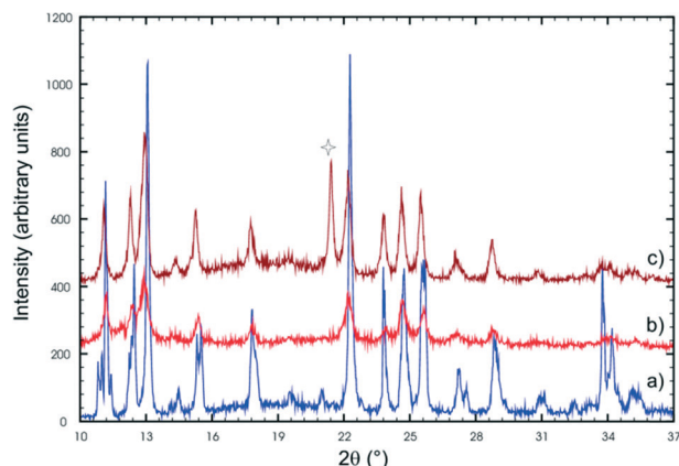
Fig. 15 X-ray powder patterns of (a) the recrystallized photodimer, and the final stage 2 photoproduct (b and c). The peak indicated by a star is due to a contaminant (probably dust as the powders were reacted in an open laboratory environment).
