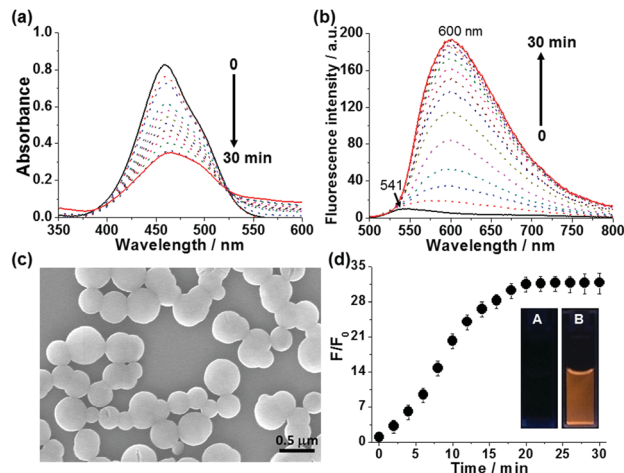
Fig. 1 Absorption (a) and fluorescence emission (b) spectra of probe 1\text{-SO}_3^- (20 \mu\text{M} ) upon incubation with spermine (20 \mu\text{M} ) for different time periods in HEPES buffer (10 mM, pH = 7.4) at 25 °C. The spectra were obtained every 2 min (0–30 min). The black solid line and red solid line indicate spectra of probe 1\text{-SO}_3^- before and 30 min after addition of spermine, respectively. Excited at 470 nm. (c) SEM image of the dried aggregates, formed from a solution of the probe 1\text{-SO}_3^- (20 \mu\text{M} ) upon 20 min incubation with spermine (20 \mu\text{M} ) in HEPES buffer (10 mM, pH = 7.4) at 25 °C. (d) Relative fluorescence intensity ( F/F_0 ) of probe 1\text{-SO}_3^- (20 \mu\text{M} ) as a function of incubation time with spermine (20 \mu\text{M} ). F and F_0 correspond to the fluorescence intensity of 1\text{-SO}_3^- in the presence and absence of spermine, respectively. The values were obtained at \lambda_{\text{em}} = 600 \text{ nm} . Inset shows photographs of probe 1\text{-SO}_3^- in the absence (A) and presence (B) of spermine after incubation for 30 min under irradiation with UV light at \lambda = 365 \text{ nm} . [1\text{-SO}_3^-] = [\text{spermine}] = 20 \mu\text{M} .
