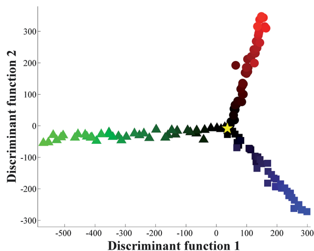
Fig. 1 PC-DFA scores plot of the FT-IR spectral data, showing the relationship between these juice samples when one of three single sugar solutions (11.7% (w/v)) are added to pure orange juice (signified by a yellow star). In this analysis PCs 1–7 were used and these account for 94.0% of the total explained variance (TEV); the averages of 4 technical replicates are plotted. The colours shading represent the level of adulteration (from 0–20%) where: fructose – black to red circles (red is highest addition of fructose); glucose – black to green triangles (green is highest addition of glucose); sucrose – black to blue squares (blue is highest addition of sucrose).
