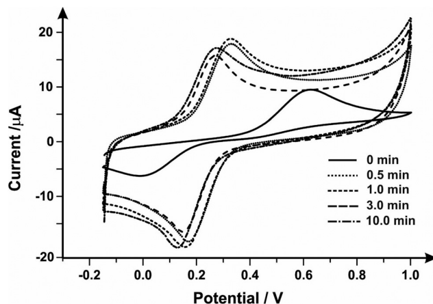
Fig. 1 Cyclic voltammetric responses obtained using a SPE in 1 \text{mmol L}^{-1} ammonium iron(II) sulfate/0.2 M \text{HClO}_4 solution as a result of varying mechanical activation/polishing times using alumina slurry. Scan rate: 50 \text{ mV s}^{-1} vs. SCE.
