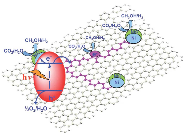
Fig. 22 Schematic of potential pathways for the transport of photo-induced electrons from a Ta 2 O 5 semiconductor nanoparticle to active CO 2 photoreduction sites mediated by graphene. Reproduced from ref. 207 with permission from The Royal Society of Chemistry.
