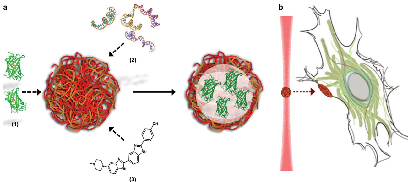
Fig. 1 The loading and delivery of coacervate microdroplets. (A) A coacervate phase comprising complexed ATP and PDPA was shown to efficiently sequester proteins (1), oligonucleotides (2) and organic molecules (3) to produce guest-loaded microdroplets. (B) A dynamic holographic assembler was used to optically-trap the microdroplets and deliver the encapsulated payload to targeted areas of the cell membrane.
