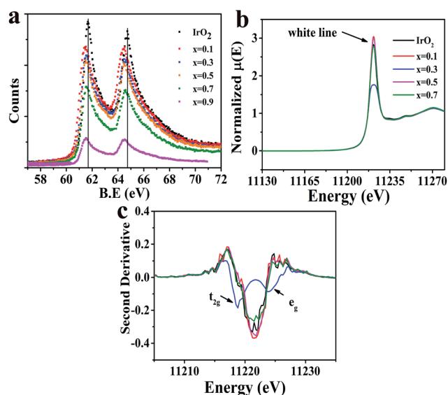
Fig. 5 (a) XPS spectra of Ir-4f in \text{Cu}_x\text{Ir}_{1-x}\text{O}_\delta compositions. The solid vertical lines correspond to the Ir-4f 7/2 and 4f 5/2 peak positions of IrO 2 . (b) Normalized Ir-L III edge XANES spectra for \text{Cu}_x\text{Ir}_{1-x}\text{O}_\delta compositions. (c) Second derivatives of Ir-L III edge XANES spectra for \text{Cu}_x\text{Ir}_{1-x}\text{O}_\delta compositions.
