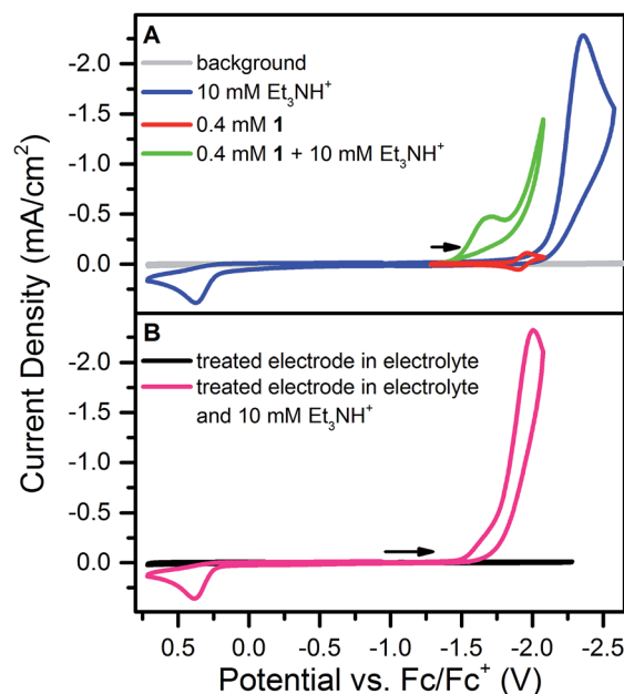
Fig. 2 (A) Cyclic voltammograms of [\text{Et}_3\text{NH}][\text{BF}_4] , 1 , and 1 plus [\text{Et}_3\text{NH}][\text{BF}_4] at 100 \text{ mV s}^{-1} in 0.25 M [\text{Bu}_4\text{N}][\text{PF}_6] . (B) Cyclic voltammograms using an electrode treated at -1.78 V for 60 s with 0.4 mM 1 and 10 mM [\text{Et}_3\text{NH}][\text{BF}_4] , rinsed, and then scanned in a solution of 0.25 M [\text{Bu}_4\text{N}][\text{PF}_6] (black line) and in a solution of 10 mM [\text{Et}_3\text{NH}][\text{BF}_4] + 0.25 M [\text{Bu}_4\text{N}][\text{PF}_6] (pink) at 100 \text{ mV s}^{-1} .
