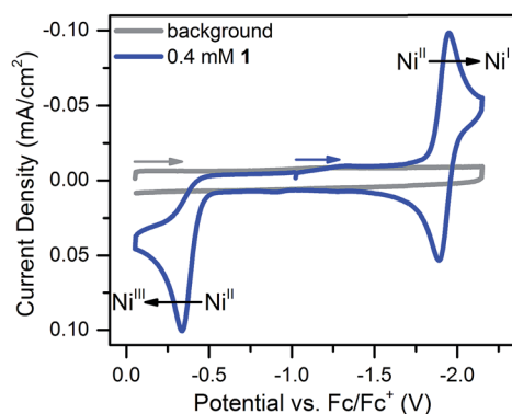
Fig. 1 Cyclic voltammogram of 0.4 mM 1 at 100 \text{ mV s}^{-1} in 0.25 M [\text{Bu}_4\text{N}][\text{PF}_6] acetonitrile solution. The \text{Ni}^{\text{II/I}} couple has an E_{1/2} of -1.92 V and the irreversible \text{Ni}^{\text{III/II}} couple has an E_{\text{p,a}} of -0.34 V.
