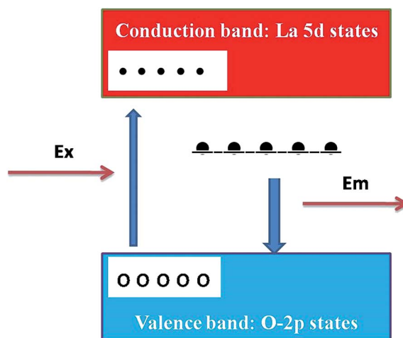
Fig. 5 Schematic model of probable mechanisms responsible for observed emission in \text{LaPO}_4 . In the schematic model, the upper (red) and the lower (light blue) bands are La 5d conduction bands and O 2p valence bands, respectively. The black bar below the conduction band corresponds to the defect level created by the oxygen deficiency. White and black circles correspond to excited holes and electrons, respectively.
