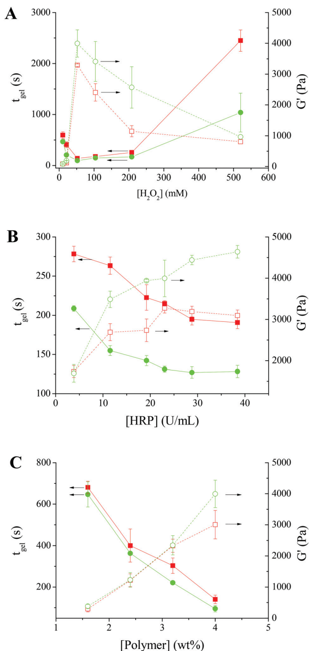
Fig. 4 (A) Influence of \text{H}_2\text{O}_2 concentration on the gelation time (solid symbols) and plateau G' (open symbols). [HRP] = 23.04 \text{ U mL}^{-1} . [Polymer] = 4 wt%. DS = 16% (■/□) or 21% (●/○). T = 37^\circ\text{C} . (B) Influence of HRP concentration on the gelation time (solid symbols) and plateau G' (open symbols). [ \text{H}_2\text{O}_2 ] = 52.0 mM. [Polymer] = 4 wt%. DS = 16% (■/□) or 21% (●/○). T = 37^\circ\text{C} . (C) Influence of polymer concentration on the gelation time (solid symbols) and plateau G' (open symbols). [ \text{H}_2\text{O}_2 ] = 52.0 mM. [HRP] = 23.04 \text{ U mL}^{-1} . DS = 16% (■/□) or 21% (●/○). T = 37^\circ\text{C} . The lines are a guide to the eye.
