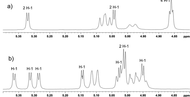
Fig. 1 Part of 1 H NMR (600 MHz) spectra showing H-1 protons of: (a) compound 2a , (b) compound 2b . Non-labeled signals belong to benzylic protons.
