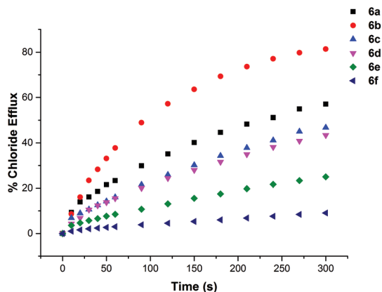
Fig. 4 Chloride efflux promoted by thioureas 6a – f (2% molar carrier to lipid) from unilamellar POPC vesicles loaded with 489 mM NaCl buffered to pH 7.2 with 5 mM sodium phosphate salts. The vesicles were dispersed in 489 mM NaNO 3 buffered to pH 7.2 with 5 mM sodium phosphate salts. At the end of the experiment, detergent was added to lyse the vesicles and calibrate the ISE to 100% chloride efflux. Each point represents the average of three trials.
