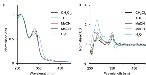
Fig. 2 Solvent effects on (a) UV-vis and (b) CD spectra of 2 . Conditions: 2 ( M_n = 1.9 \times 10^4 g mol -1 , M_w = 2.7 \times 10^4 g mol -1 ), 25 °C, path length = 1 mm. UV spectra were normalised at 270 nm. CD spectra were normalised as that the absorbance at 270 nm is 1.0.
