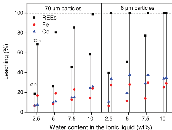
Fig. 7 Leaching (%) of Co, Fe and REEs (Nd + Dy) from two different milled roasted NdFeB magnets ( \approx 70 \mu m and 6 \mu m). The leaching is shown as function of time (24 and 72 h) and as function of the water content in the ionic liquid (2.5, 5, 7.5 and 10 wt%). The solutions were stirred 600 rpm at 90 ^{\circ} C.
