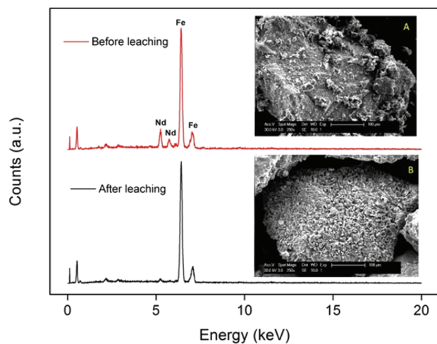
Fig. 5 SEM images (magnified 250 \times ) and EDX spectrum of the surface of the large NdFeB particles ( \approx 300 \mu m) before (A) and after (B) leaching.
