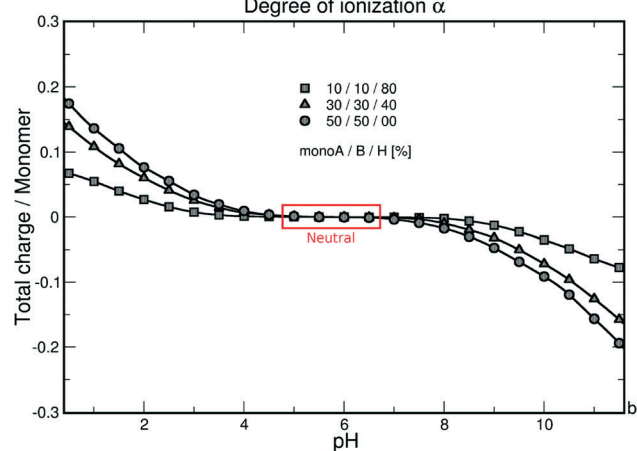
Fig. 1 (a) Monte Carlo titration curves calculated as a function of the degree of ionization \alpha , and (b) total charge per monomer as a function of pH of a weak random chain surrounded by monovalent counterions. The deprotonation of monomers A (or B) is promoted by the presence of charged monomers B (or A), and is more efficient in the case of strong attractive electrostatic interactions without hydrophobic monomers (0% monoH). Titration curves exhibit an intermediate pH range where chains are globally neutral with all monomers A and B charged.
