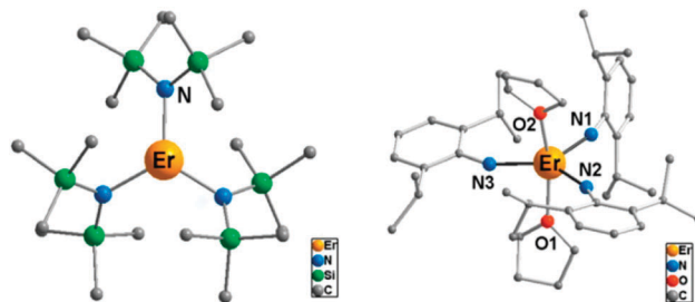
Fig. 6 Molecular structures of the complexes [\text{Er}(\text{N}(\text{SiMe}_3)_2)_3] (left) and [\text{Er}\{\text{NHPh}^1\text{Pr}_2\}_3(\text{THF})_2] (right), with hydrogen atoms omitted for clarity. Adapted with permission from ref. 22. Copyright 2014 American Chemical Society.
