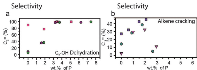
Fig. 14 Effect of weight loading of phosphorus on (a) dehydration of ethanol and selectivity for ethylene at temperatures > 400 °C. \blacksquare = Zhang et al. 77 \blacksquare = Ramesh et al. 81 \blacksquare = Ramesh et al. 84 Differences between reaction temperature, Si/Al ratio, crystal size and space velocity have not been taken into account. (b) Alkene cracking and selectivity for propylene (%). \blacksquare = Zhao et al. 64 \blacksquare = Xue et al. 57 \blacksquare = Xue et al. 79 Differences between reaction temperature, Si/Al ratio, crystal size and space velocity have not been taken into account.
