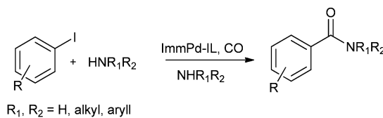
Scheme 33 Reagents and conditions: aryl iodide (1 mmol), amine (2 mmol), ImmPd-IL (2 mol%), \text{Et}_3\text{N} (3 mmol), toluene (10 mL), CO pressure (1 MPa), temp. 100^\circ\text{C} , time 8 h.
