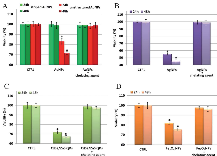
Fig. 5 Toxicity assessment of different types of NPs in the absence/presence of specific ion chelators. WST-8 proliferation assays upon treatment with (A) striped and unstructured AuNPs (20 nM), (B) AgNPs (2 nM), and (C) CdSe/ZnS QDs (5 nM) in HeLa cells in the presence of 2,3-dithiopropanol (BAL); HeLa cells were pretreated for 30 min with/without 1 μM BAL and then exposed to the NPs for 24–48 h. (D) Proliferation assay upon treatment with 2.5 nM of Fe 3 O 4 NPs. In this case, HeLa cells were pretreated for 30 min with/without 100 μM desferrioxamine (dfx) and then exposed to Fe 3 O 4 NPs for 24–48 h. In all cases, the pretreatment with chelating agents suppresses, almost totally, the toxicity of the NPs. CTRL represents the negative control; values are mean ± SD. Differences between treated samples and controls ( n = 8 ) were considered statistically significant for *P < 0.05 and non-significant for P > 0.05 .
