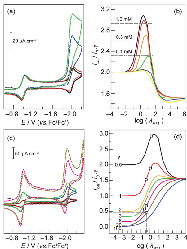
Fig. 3 (a) CVs of a 0.1 mM solution of 3 in the absence of benzoic acid (—) and in the presence of 0.05 (•••••), 0.3 (—), and 0.6 (—•) mM benzoic acid. Scan rate, 30 mV s -1 ; 0.2 M TBAPF 6 in acetonitrile. Glassy carbon working electrode, Ag/AgNO 3 reference electrode, and Pt wire counter electrode. (b) Working curves generated by simulating CVs with \gamma = 0.5 and \rho = 100 (—), 10 (—), 1 (—), 0.1 (—), 0.01 (—), and 0.001 (—). Horizontal lines indicate normalized current values ( i_{cat}/i_0\gamma ) obtained at the designated porphyrin concentrations, with half an equivalent of benzoic acid. (c) CVs of 0.1 (—), 0.3 (—), and 1 mM (—) solutions of 3 in the absence of benzoic acid and in the presence of 0.05 (•••••), 0.15 (—•), and 0.5 (—•) mM benzoic acid, respectively. Scan rate, 30 mV s -1 ; 0.2 M TBAPF 6 in acetonitrile. Glassy carbon working electrode, Ag/AgNO 3 reference electrode, and Pt wire counter electrode. (d) Working curves generated by simulating CVs with \rho = 10 . Experimental data points for 3 (□) and 2 (○) acquired at scan rates of 30 and 100 mV s -1 respectively.
