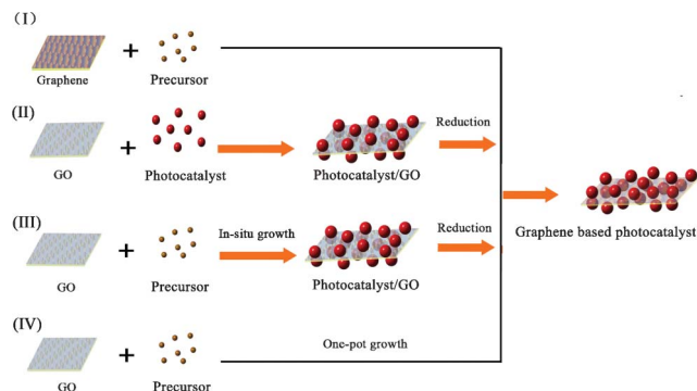
Fig. 3 Four synthetic strategies for the fabrication of graphene-based photocatalysts.
