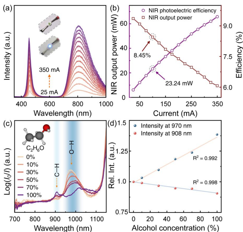
Fig. 4. (a) Electroluminescence spectra of NIR pc-LED device under different driving currents (25 mA -350 mA). The insets show a fabricated device with (up) and without (below) LED on; (b) NIR output power, and NIR photoelectric conversion efficiency of the fabricated NIR pc-LED device; (c) Calculated absorption spectra of the alcohol in various concentrations; (d) Relationships between intensity ratio (at 908 nm and 970 nm) and alcohol concentrations.
