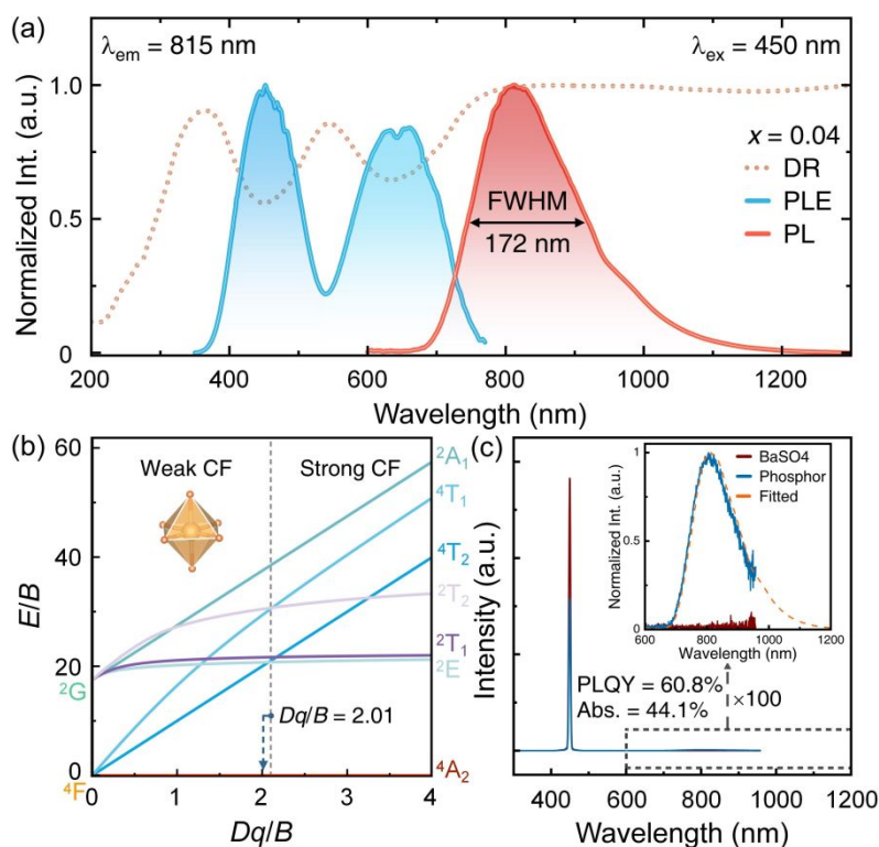
Fig. 2. (a) DR (orange dotted line), PLE (blue), and PL (red) spectra of \text{Mg}_{2.96}\text{Gd}_2\text{Ge}_3\text{O}_{12}:0.04\text{Cr}^{3+} phosphor excited by 450 nm radiation and monitored at 815 nm wavelength; (b) Tanabe-Sugano diagram for \text{Cr}^{3+} ion in octahedral crystal field; (c) Photoluminescence quantum yield and absorption efficiency of \text{Mg}_{2.96}\text{Gd}_2\text{Ge}_3\text{O}_{12}:0.04\text{Cr}^{3+} phosphor excited by 450 nm.
