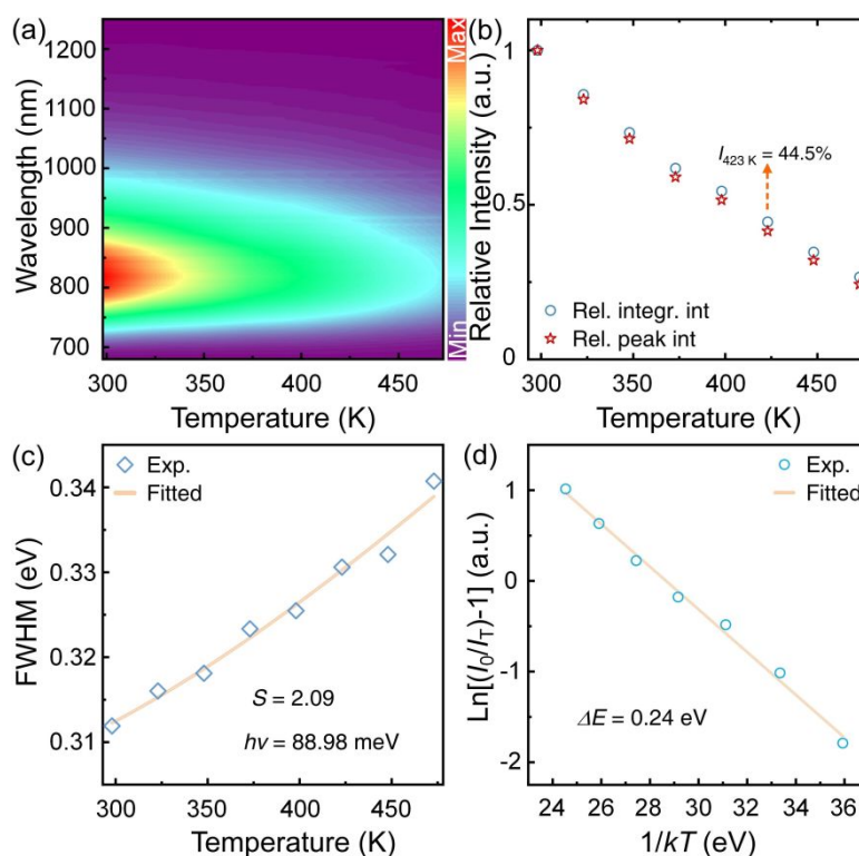
Fig. 3. (a) Contour plot of the temperature-dependent emission spectra, and (b) Relative integral and peak intensity of \text{Mg}_{2.96}\text{Gd}_2\text{Ge}_3\text{O}_{12}:0.04\text{Cr}^{3+} phosphor excited by 450 nm; (c) Fitted Huang-Rhys factor ( S ) and the phonon energy ( h\nu ); (d) Fitting the relationship between \text{Ln}[(I_0/I_T)-1] versus 1/kT .
